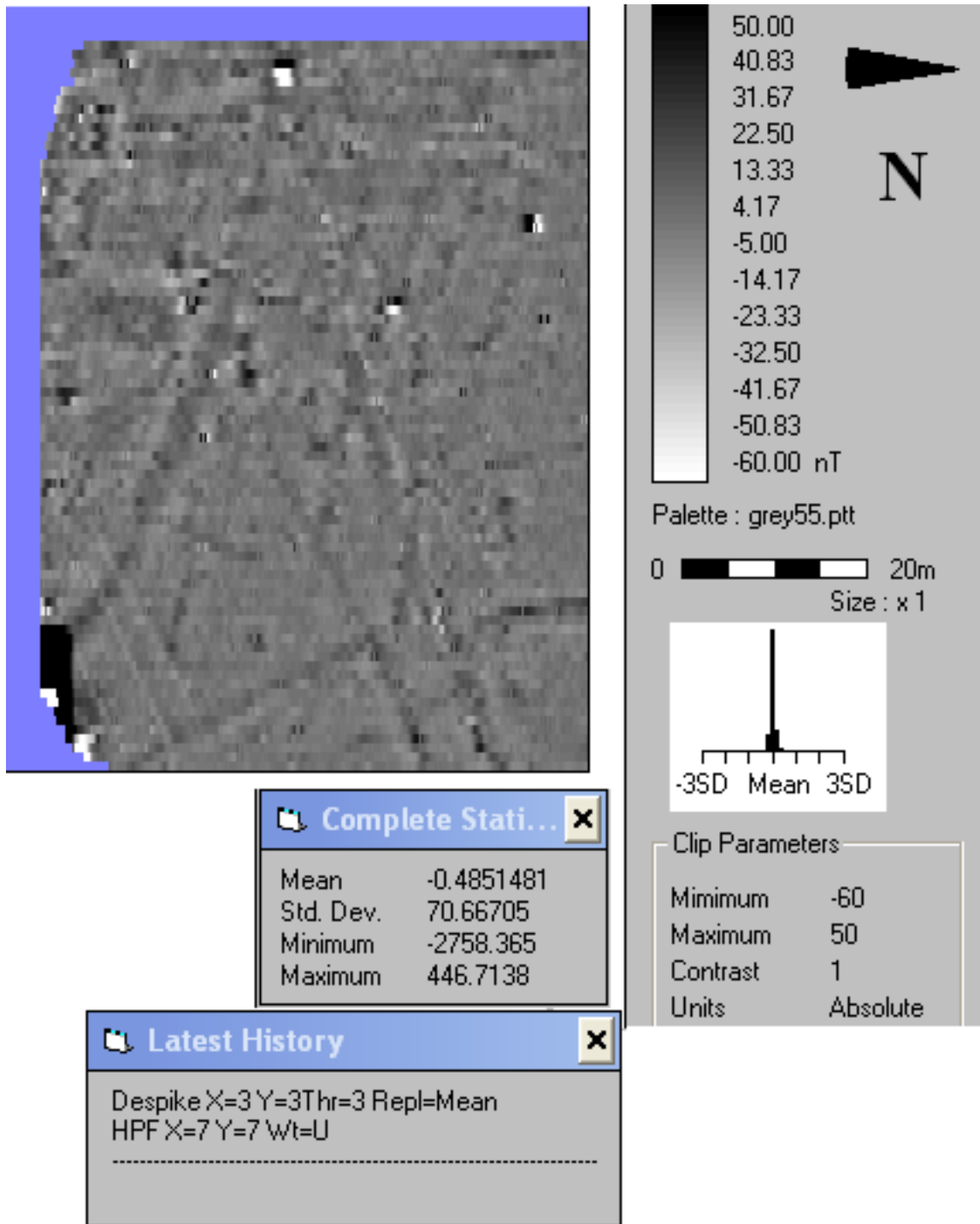
Figure 16a Glebe Field magnetometer results: processed data, grey-scale plot
